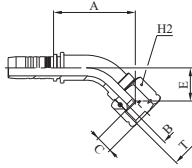
M22542 45° JIC FEMALE SWEPT ELBOW 37° CONE SEAT - SAE J516 / ISO 12151-5 (THRUST-WIRE NUT)
