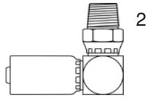
Hose x MNPT SW 90 DEG Elbow Crimp Fitting
