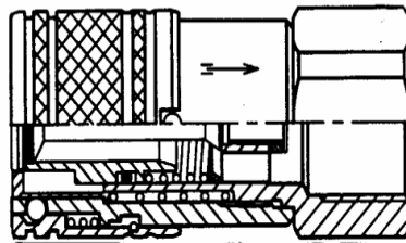
FEMALE BODY STEEL
