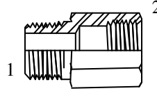
Male BSPP x Female BSPP Extended Bushing
