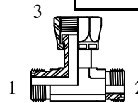
Male BSPP x Female BSPP Swivel Branch Tee
