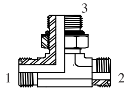
Male BSPP x Male BSPP Adjustable Branch Tee C/W Retaining Ring/O-Ring
