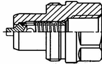
MALE TIP STEEL
