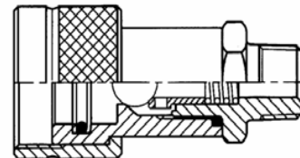
FEMALE BODY STEEL
