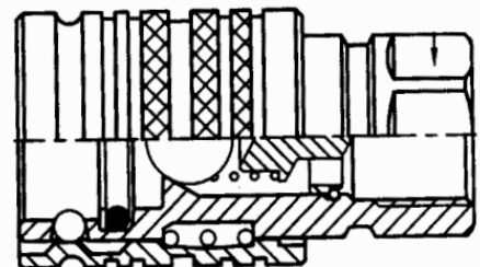
FEMALE BODY STEEL BALL TYPE
