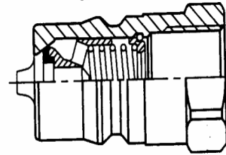
MALE TIP PINE DECOMPRESION CONECT UNDER PRESSURE S71-4PB
