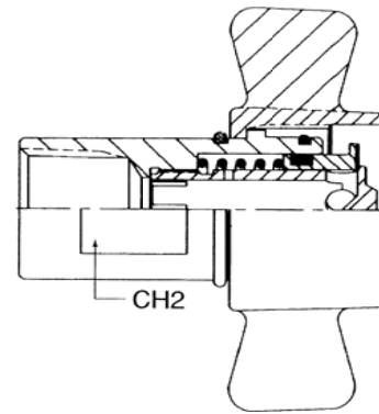
BRASS COUPLER
